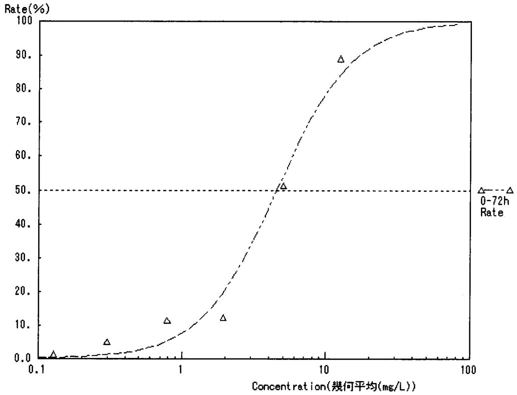
Dose-response curve for EC50 of Algae Growth Test (Logit method) 98839
