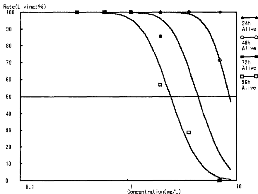
Dose-response curve for LC50 of Fish Acute Toxicity Test JCL048128 (Probit method)
